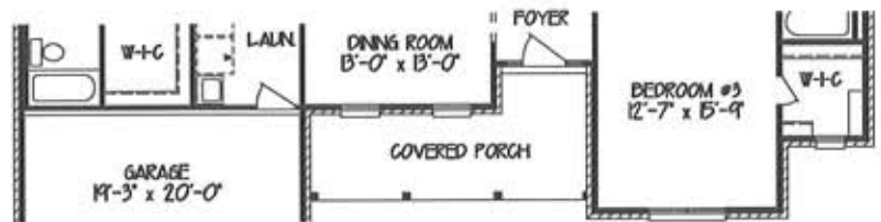
OPTIONAL FLOOR PLAN 'B' (INCL. FULL FRONT PORCH, 2' ADDED @ BDRM #3 FRONT & UPGRADED DBL. GABLE FRONT) ADDS 28 SF
